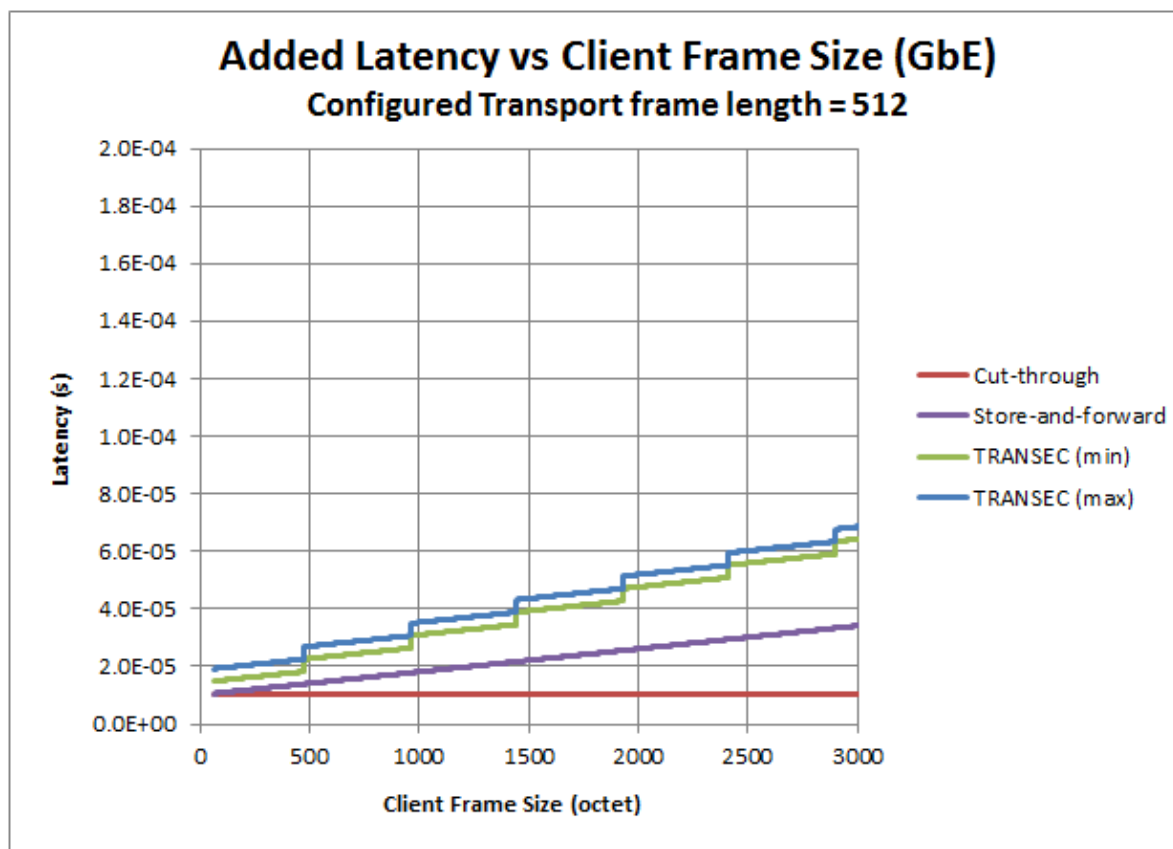
Figure 29. Latency variation with transport length of 512 octets
