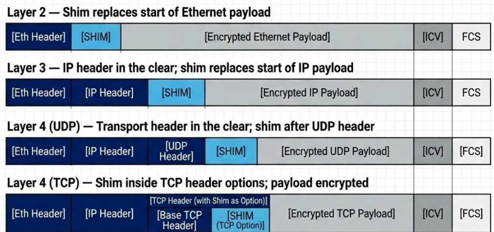
Figure 31. TIM encrypted frame formats by encryption layer
