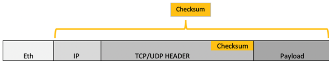
Figure 35. Layer 4 checksum calculation
