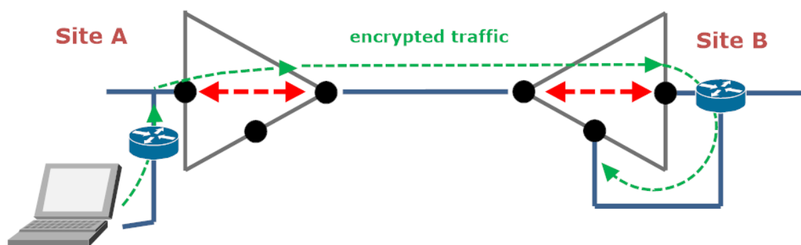
Figure 16. In-line management
