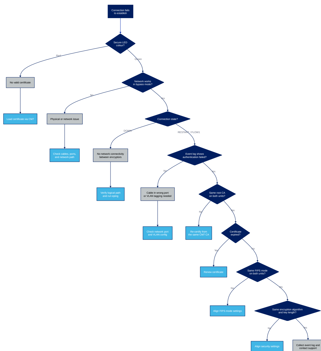
Figure 44. Connection establishment diagnostic flowchart
