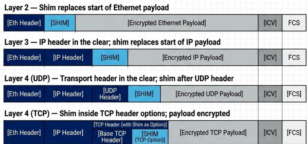
Figure 28. TIM encrypted frame formats by encryption layer
