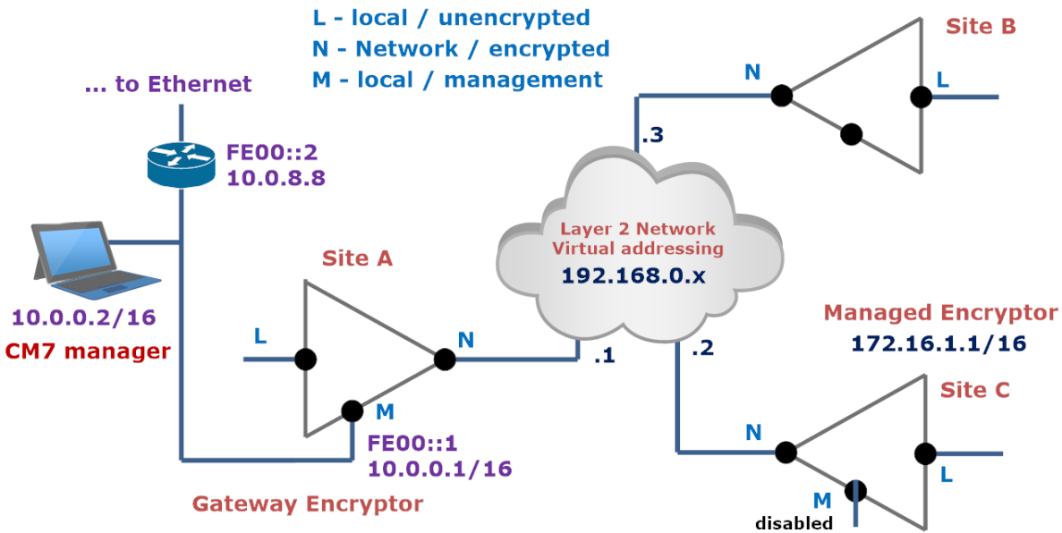
Figure 15. Inband management configuration example
