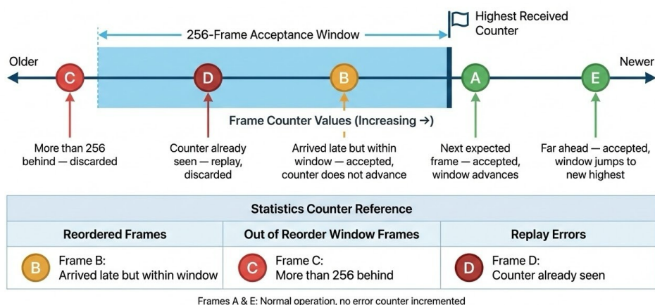
Figure 21. Replay protection: 256-frame sliding acceptance window
