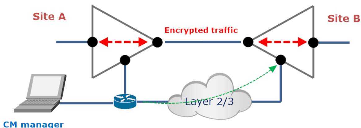
Figure 13. Out-of-band management
