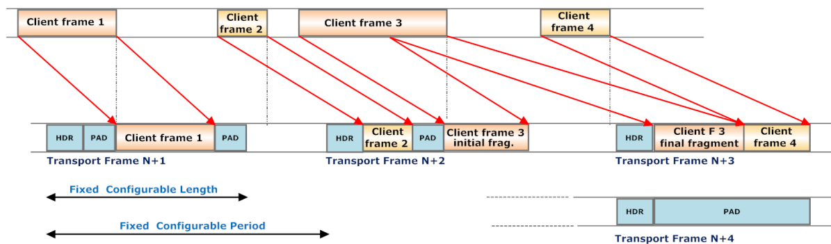
Figure 25. TRANSEC frame assembly
