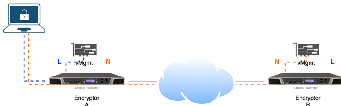
Figure 17. Virtual management
