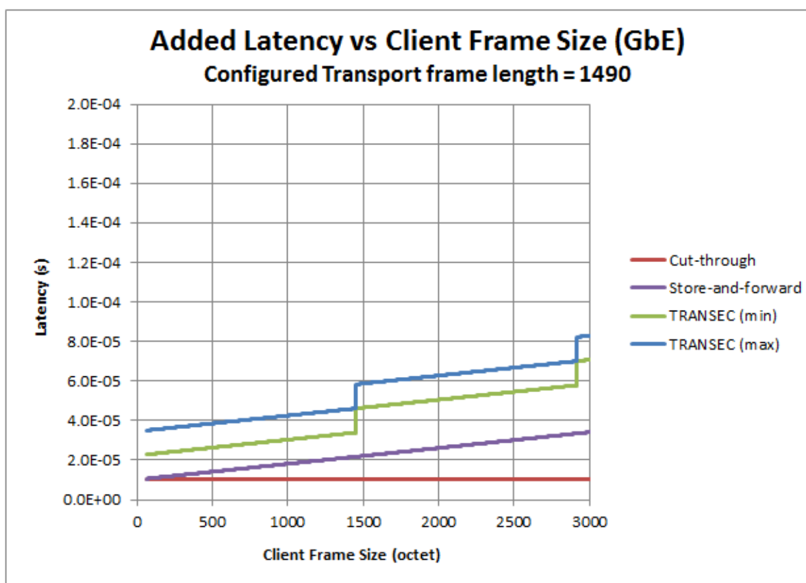
Figure 27. Latency variation with transport length of 1490 octets
