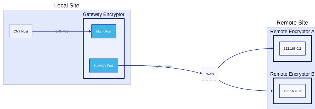
Figure 17. In-band management architecture
