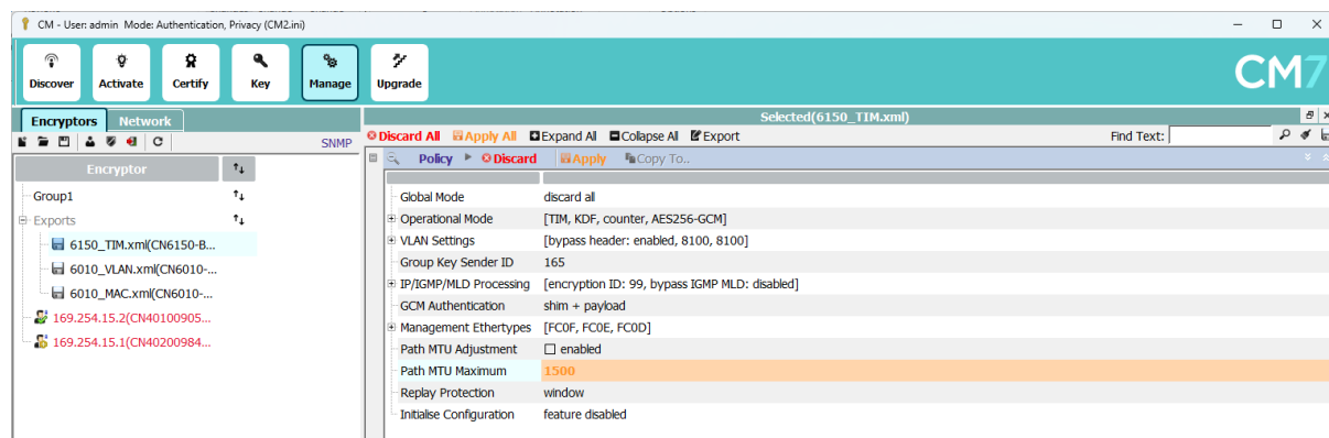
Figure 26. PMTUM configuration
