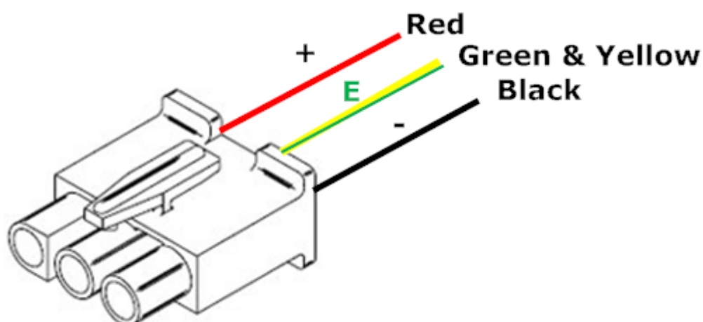
Figure 6. Molex pin connections
