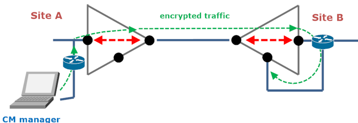
Figure 19. In-line management
