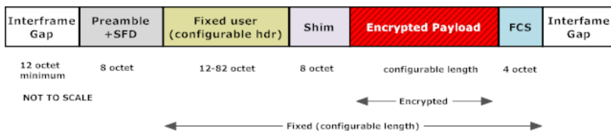
Figure 27. TRANSEC frame
