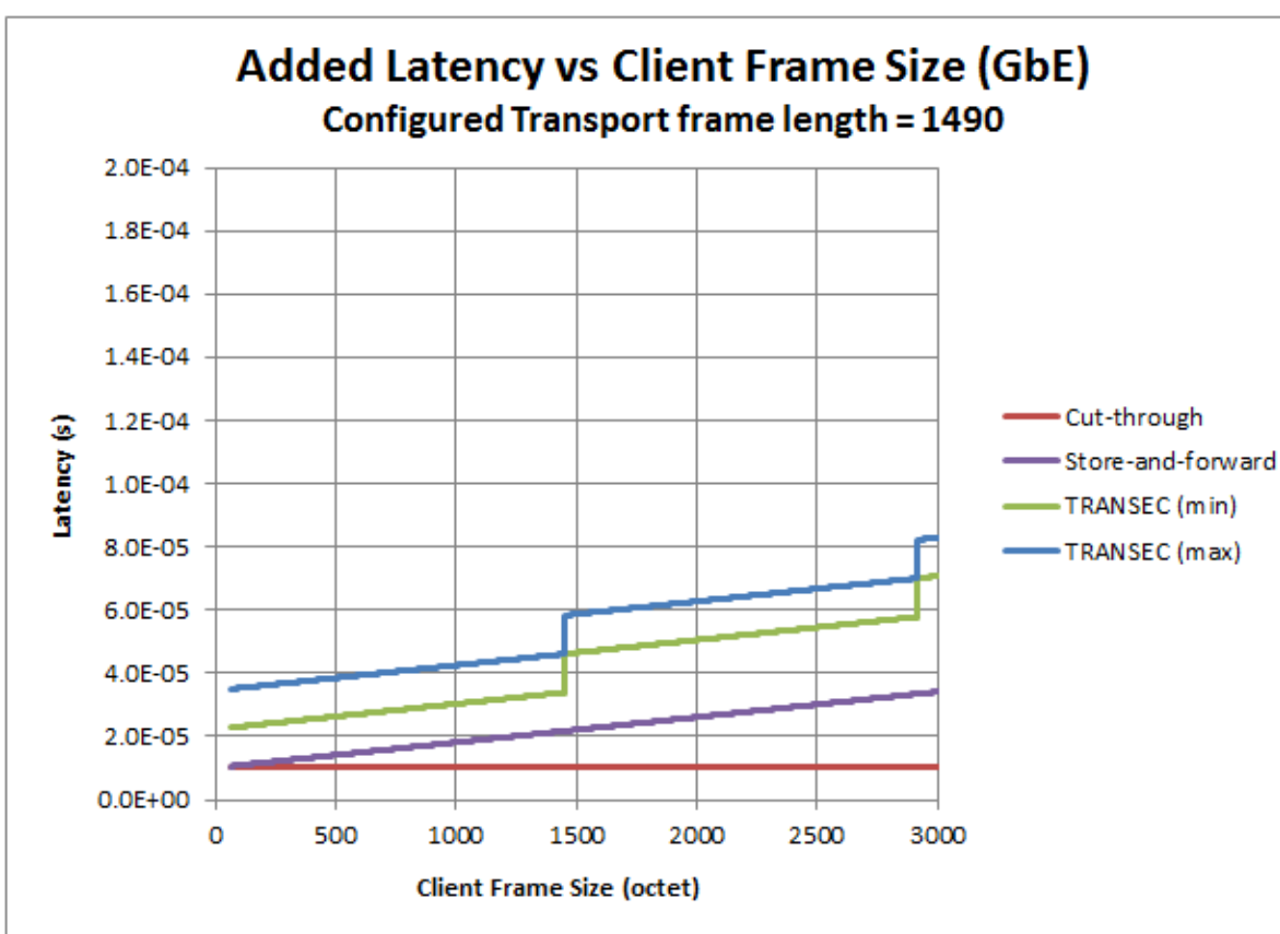
Figure 31. Latency variation with transport length of 1490 octets
