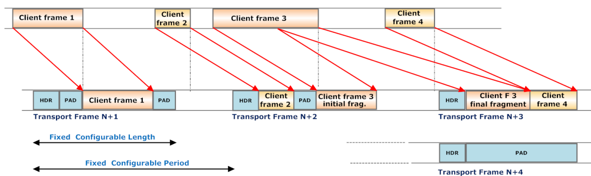
Figure 29. TRANSEC frame assembly
