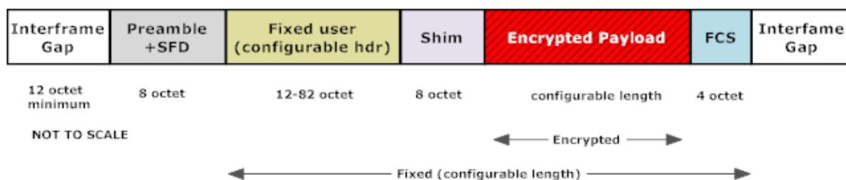
Figure 28. TRANSEC frame
