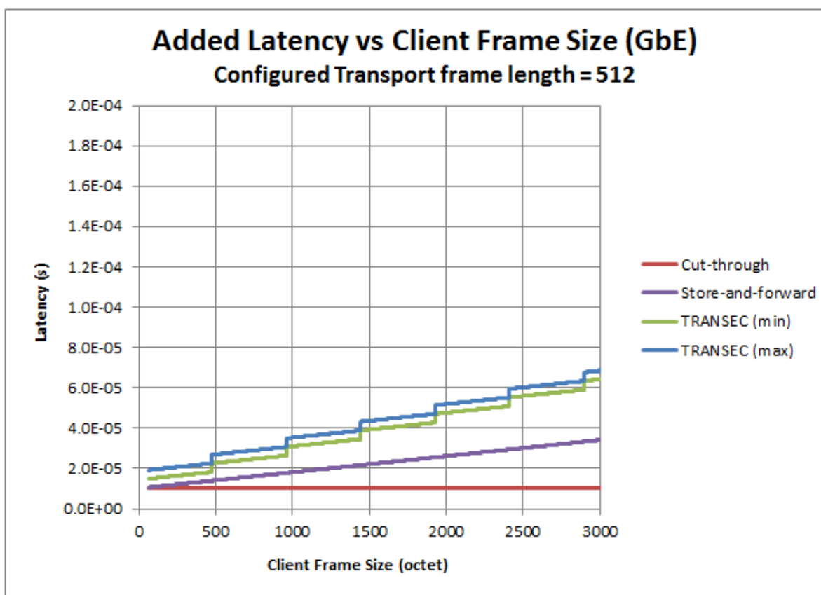
Figure 30. Latency variation with transport length of 512 octets
