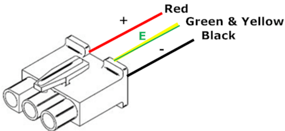
Figure 7. Molex pin connections
