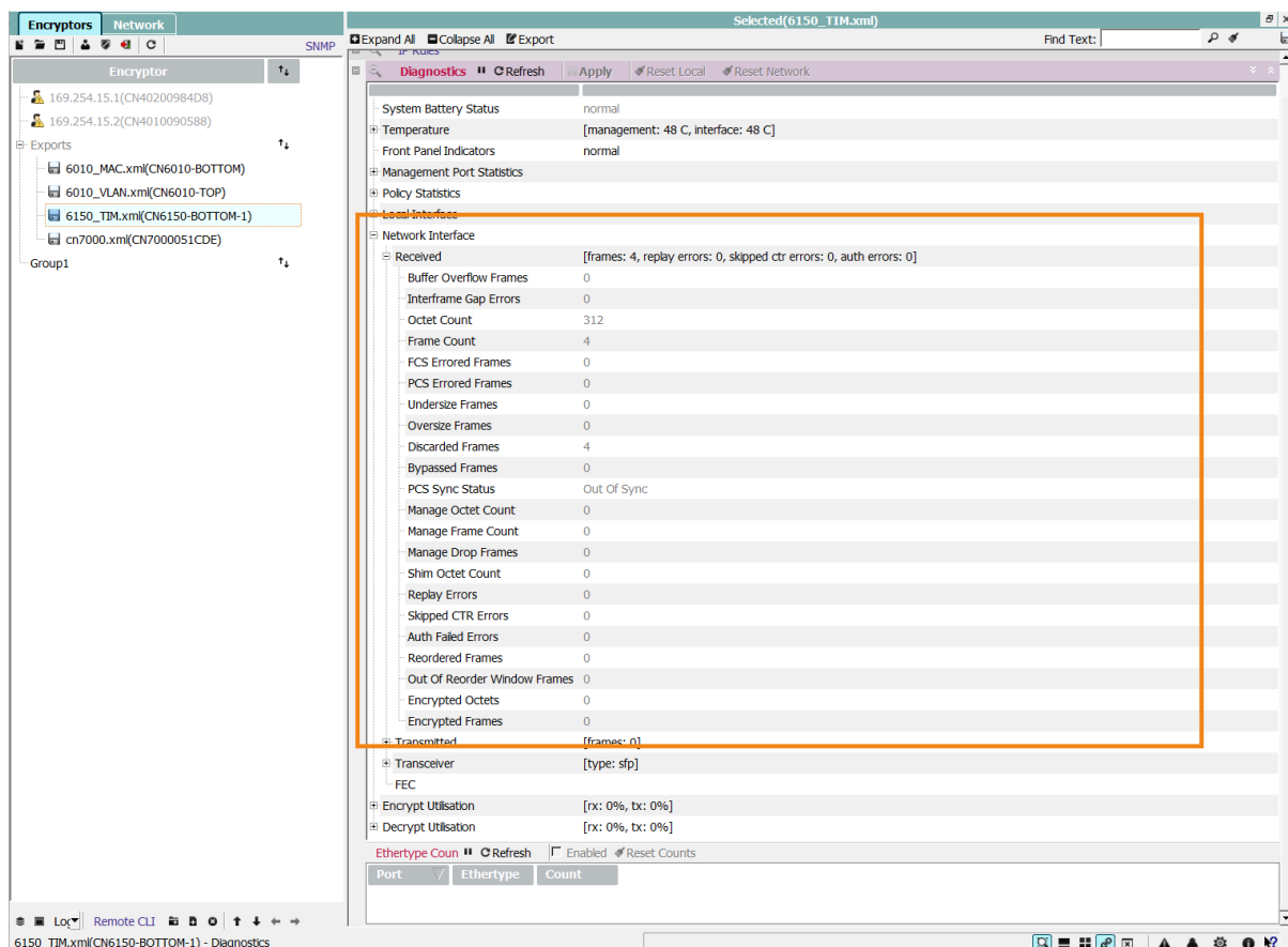
Figure 42. Network interface diagnostics — Rx statistics
