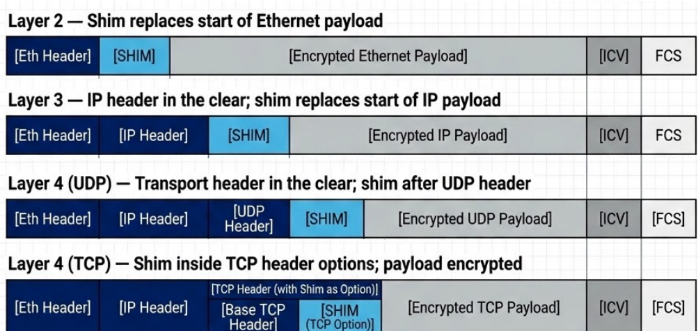
Figure 32. TIM encrypted frame formats by encryption layer
