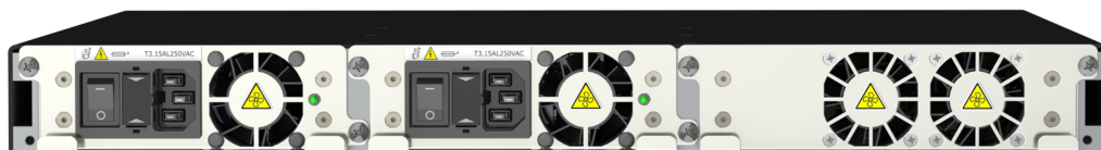
Figure 5. CN6140 Rear view
