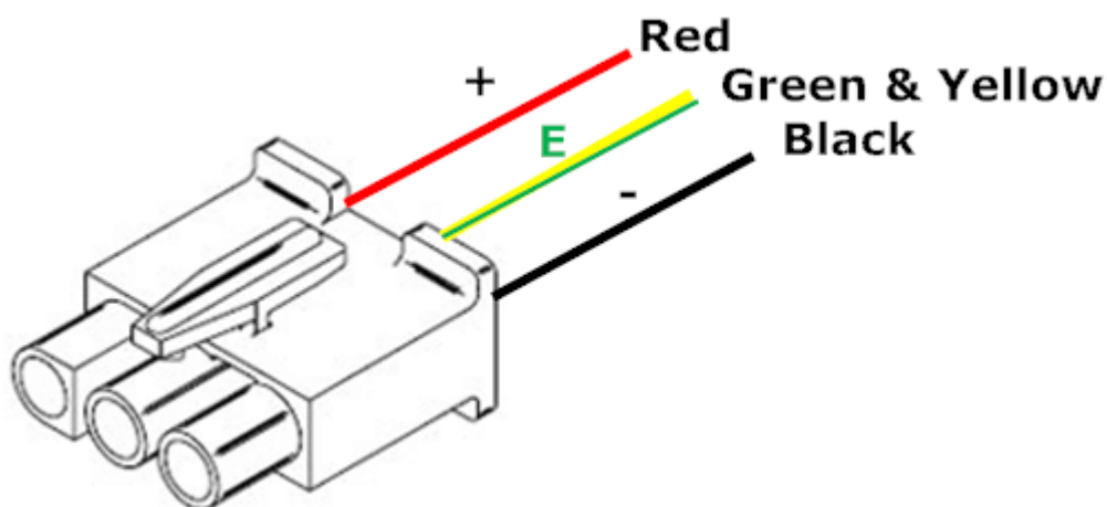
Figure 6. Molex pin connections
