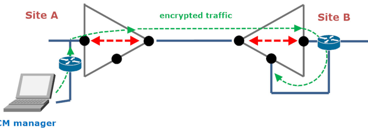
Figure 19. In-line management
