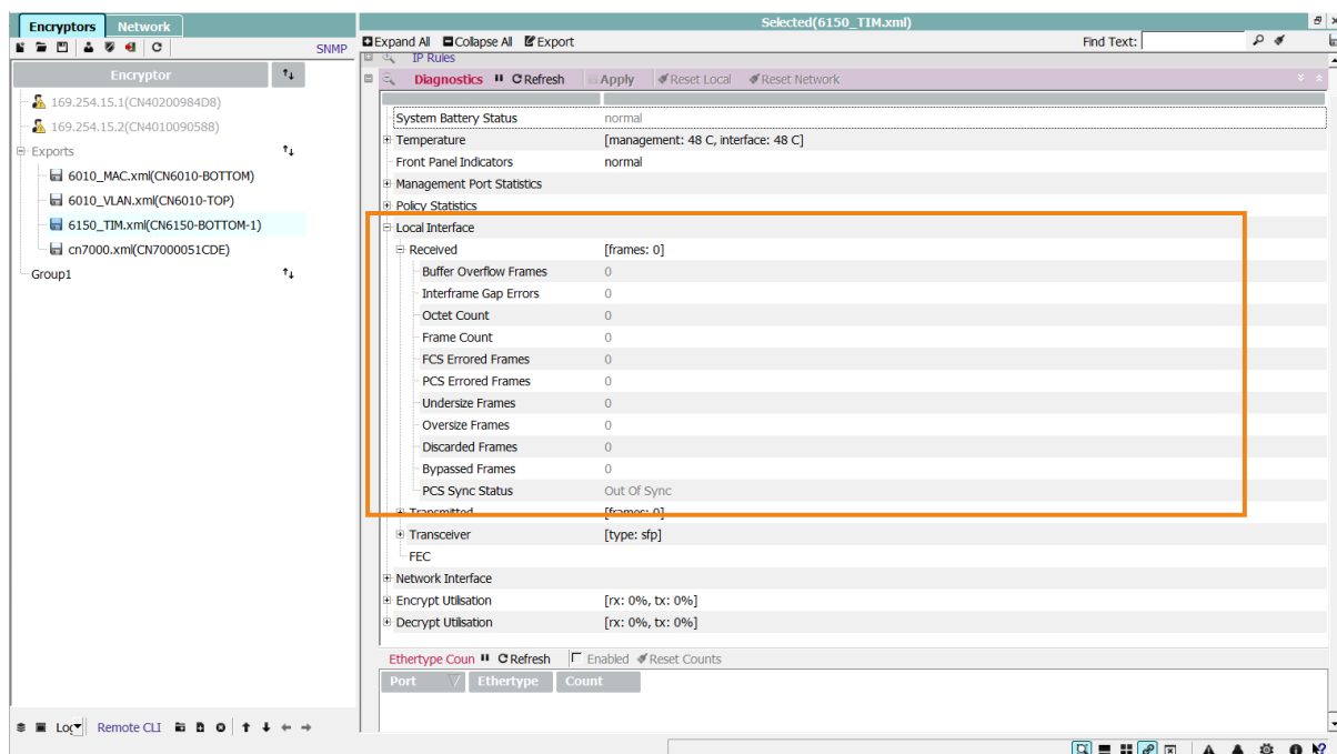
Figure 31. Local interface diagnostics — Rx statistics
