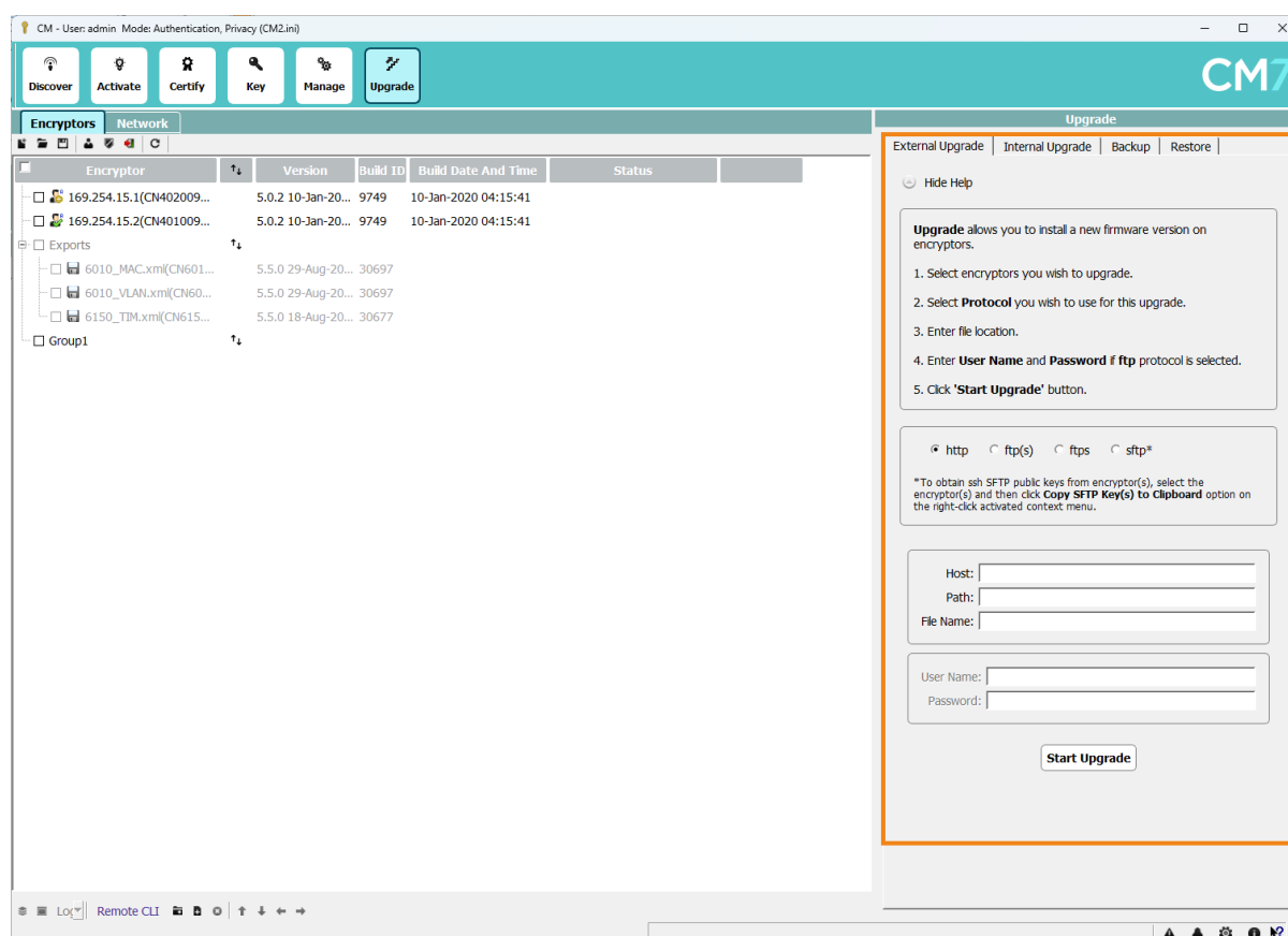
Figure 36. External upgrade dialog
