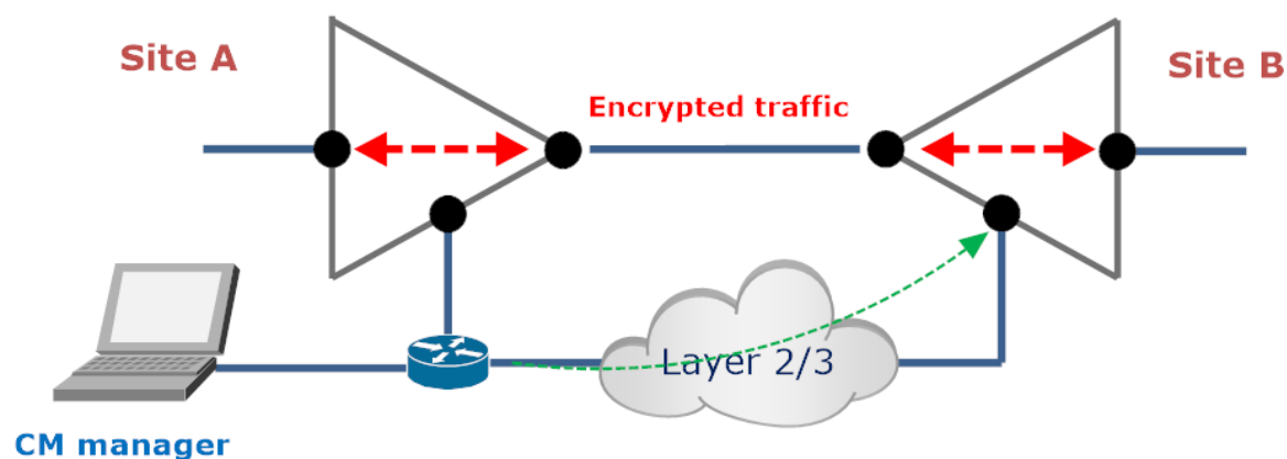
Figure 16. Out-of-band management
