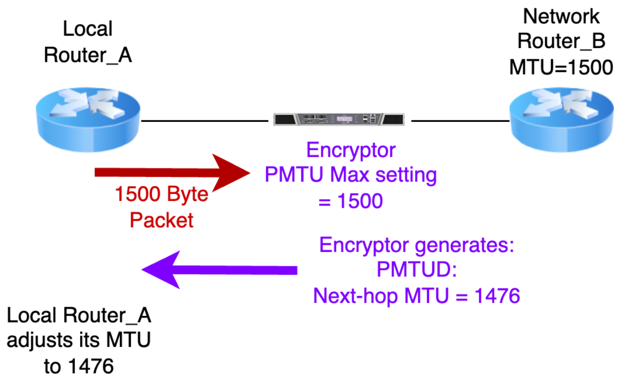
Figure 25. PMTU Max operation
