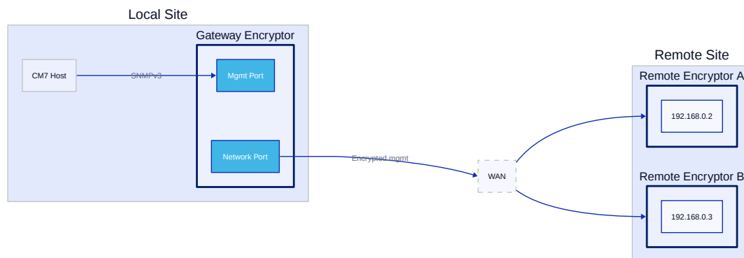
Figure 17. In-band management architecture
