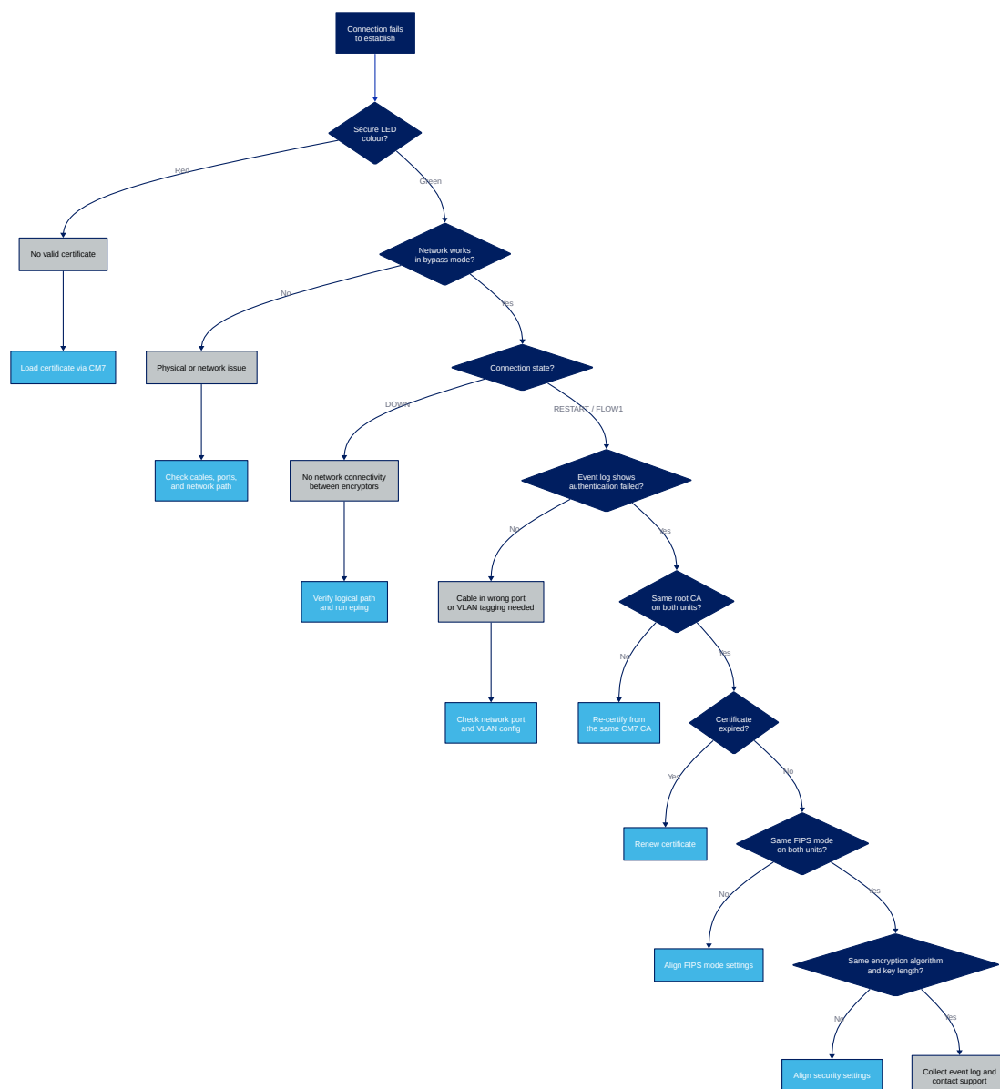
Figure 38. Connection establishment diagnostic flowchart
